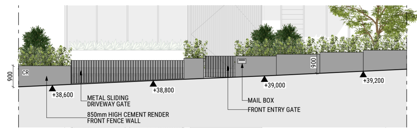
FRONT FENCE ELEVATION 1:100
